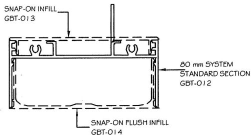
ASSEMBLY DETAIL SCALE 1:2
