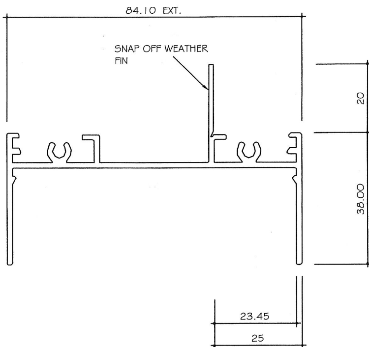
80 mm SYSTEM - STANDARD SECTION
