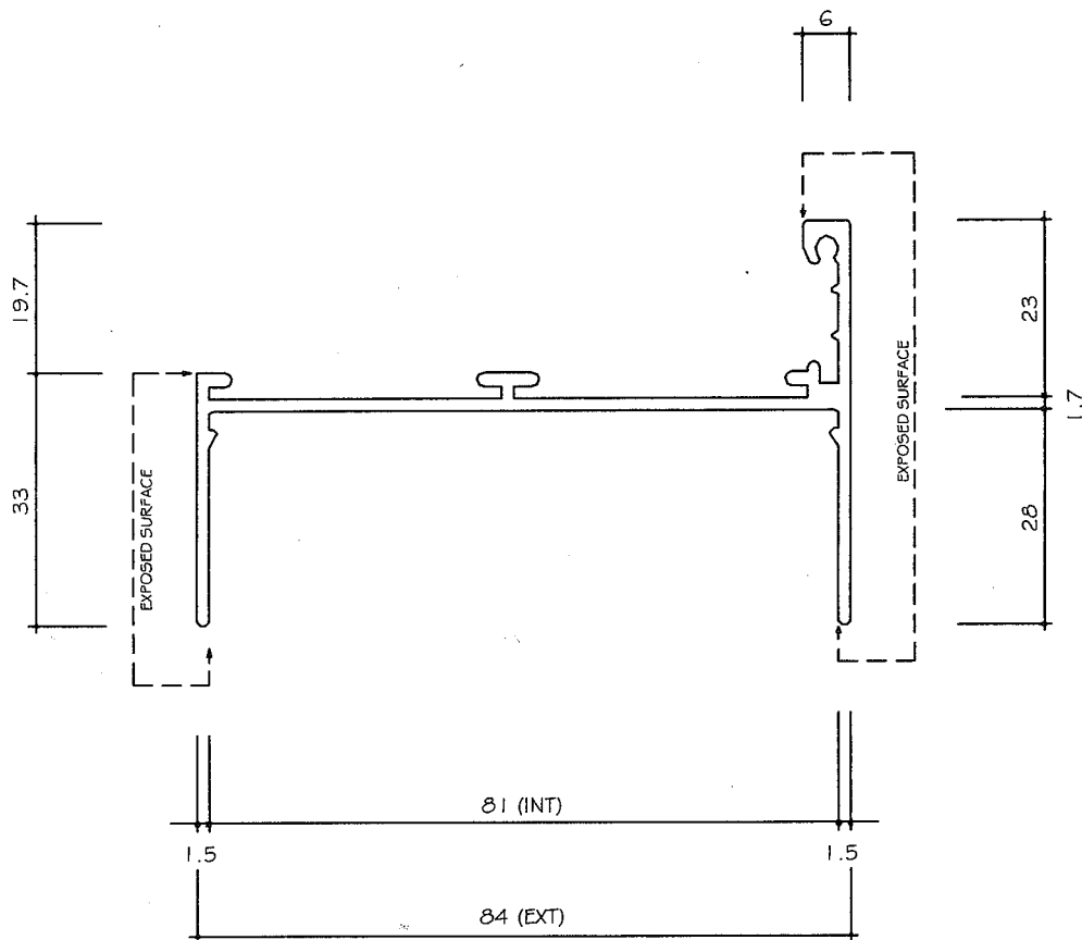
ASSEMBLY DETAIL SCALE 1:2
