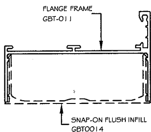
ASSEMBLY DETAIL SCALE 1:2
