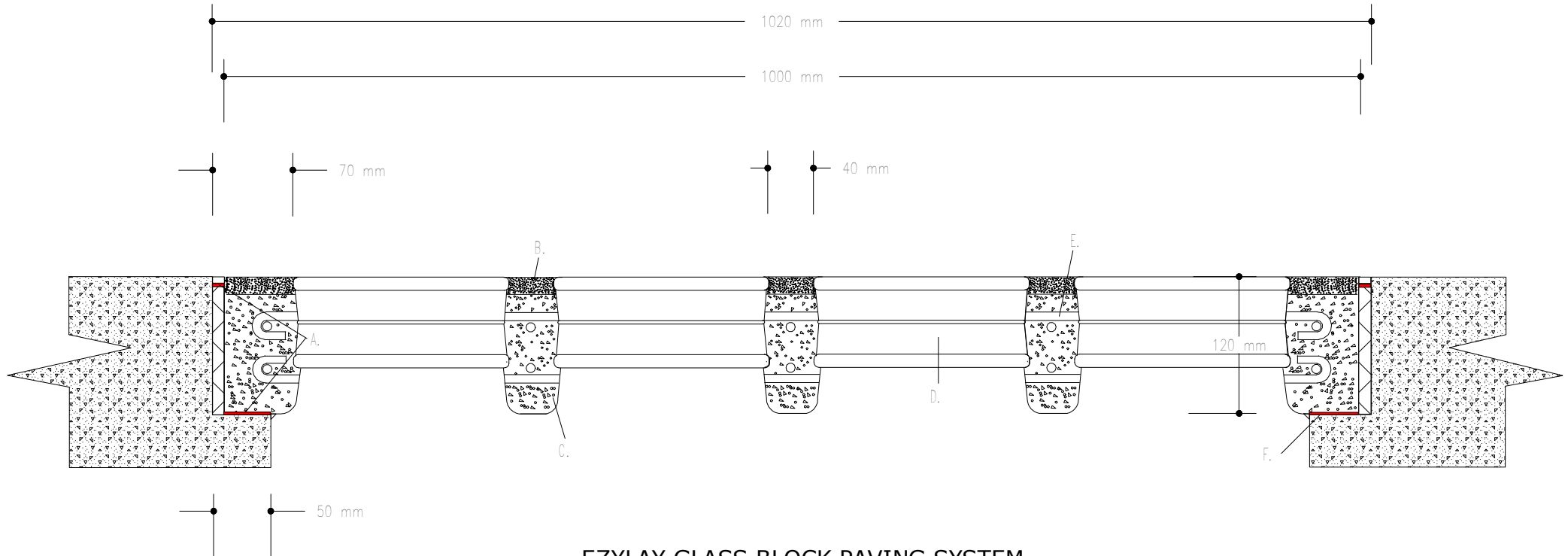
EZYLAY GLASS BLOCK PAVING SYSTEM SECTION DETAIL BG 198 -190 x 190 x 80mm PAVERS
